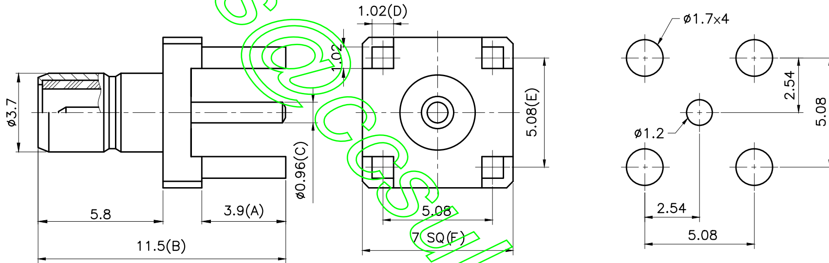
PCB MOUNTING HOLE
