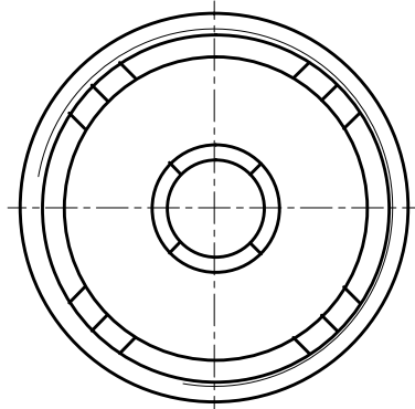
UHF FEMALE
