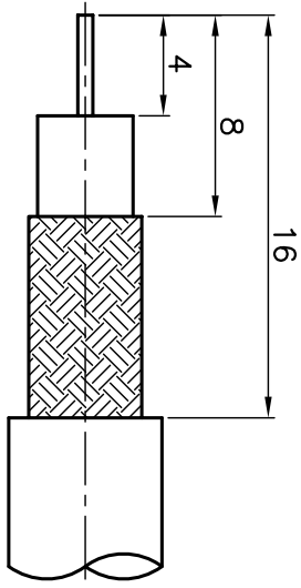
RECOMMENDED CABLE STRIPPING DIM'S
