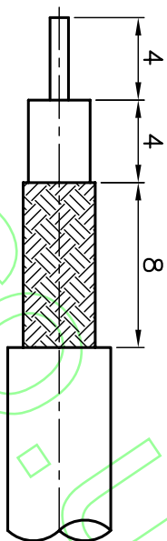
CABLE STRIPPING DIM'S
