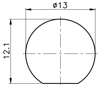
PANEL HOLE
